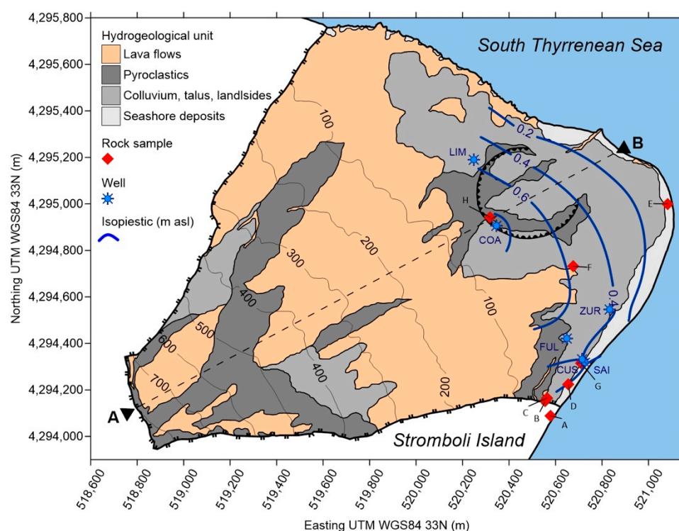
Figure 2. Detailed map of the studied area reporting the location of water wells and rock samples for the hydraulic conductivity determinations, main hydrogeological divide, limits of the hydrogeological units, and isopiestic lines (contour interval 0.2 m a.s.l.); elevations are in m a.s.l. The dashed line A–B indicates the trace of the hydrogeological section later discussed.
