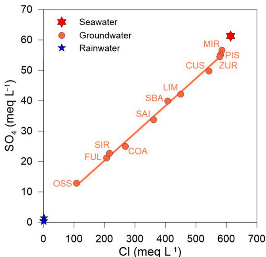
Figure 6. Cl vs. \text{SO}_4 diagram reporting the values for groundwater, rainwater (two sampling sites) [24], and seawater [11] of Stromboli Island.
