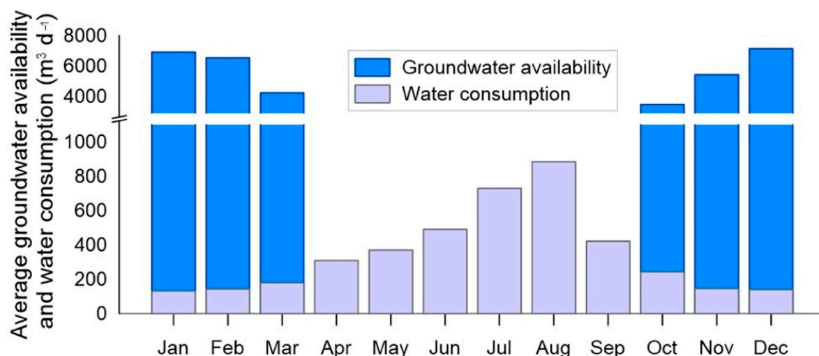
Figure 11. Comparison between the monthly average values of groundwater availability and water consumption [24].
