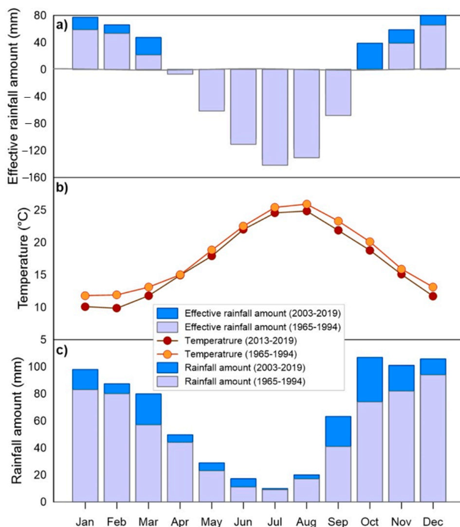
Figure 3. Hydrological balance. Monthly variation of effective rainfall amount (a), air temperature (b), and rainfall amount (c) at Stromboli.
