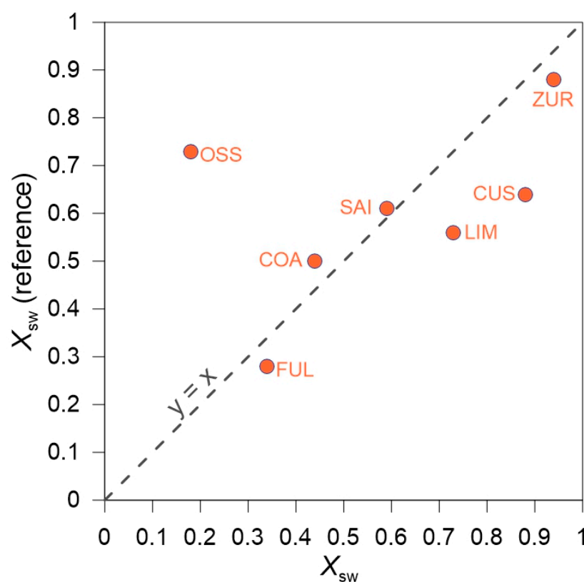
Figure 7. The fraction of seawater ( X_{sw} ) calculated using the Cl concentration of samples taken under dynamic conditions (this study) plotted versus the fraction calculated from samples taken under static conditions [11].
