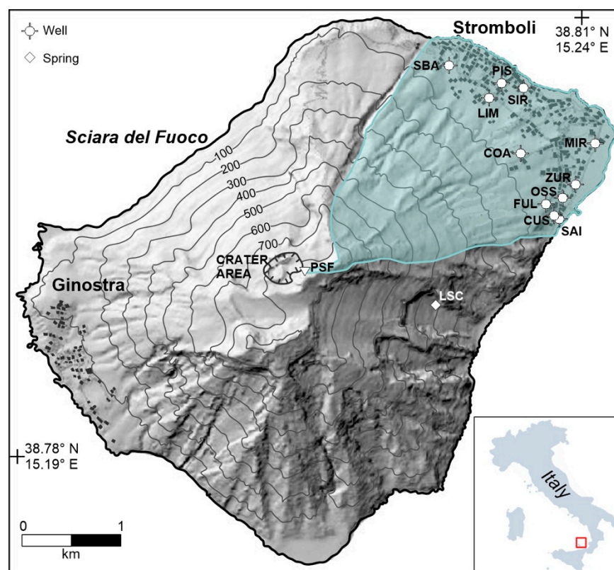
Figure 1. Map of Stromboli Island showing the study area (shaded polygon) and the location of water wells (circles), a spring (diamond), and rain collectors (triangles).
