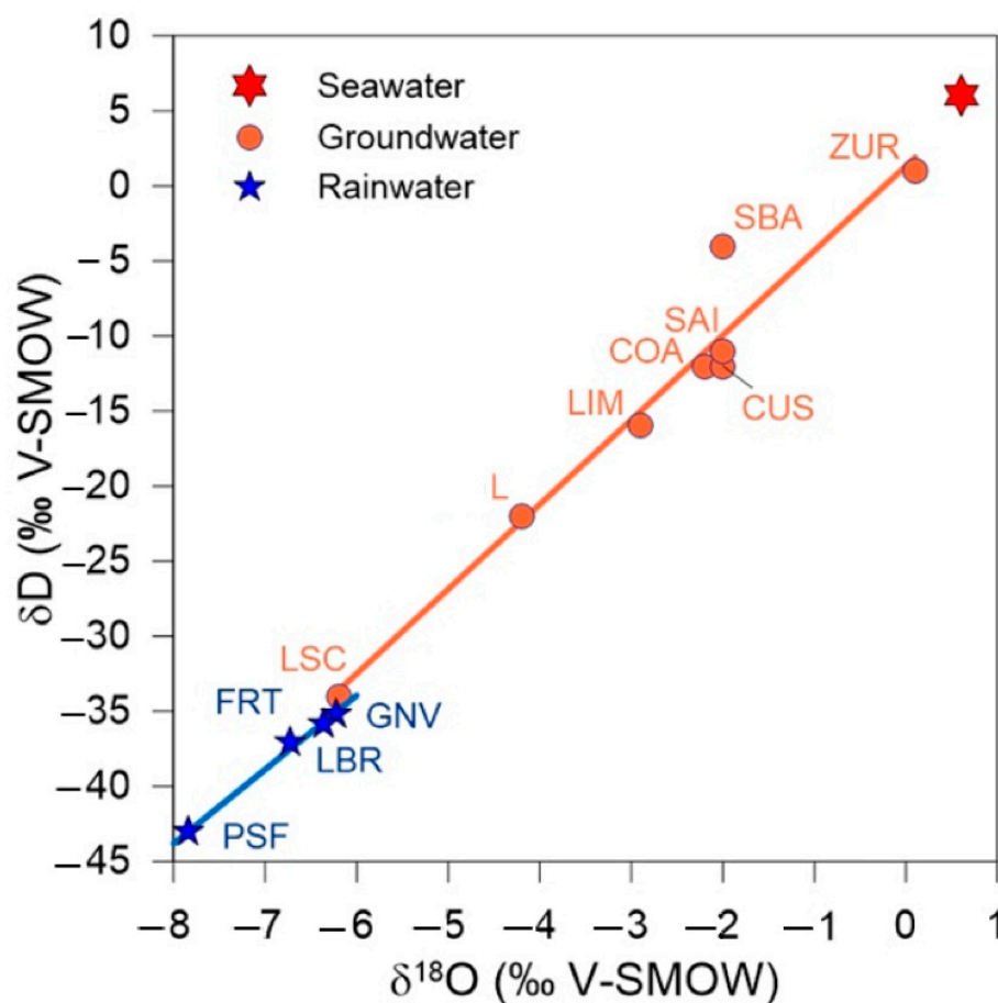
Figure 9. \delta^{18}\text{O} vs. \delta\text{D} diagram reporting the isotopic composition of the groundwater [11], rainwater [19], and seawater [11] of Stromboli Island. The blue line is the best fit of the rain compositions, and the orange one is the best fit of the groundwater samples.
