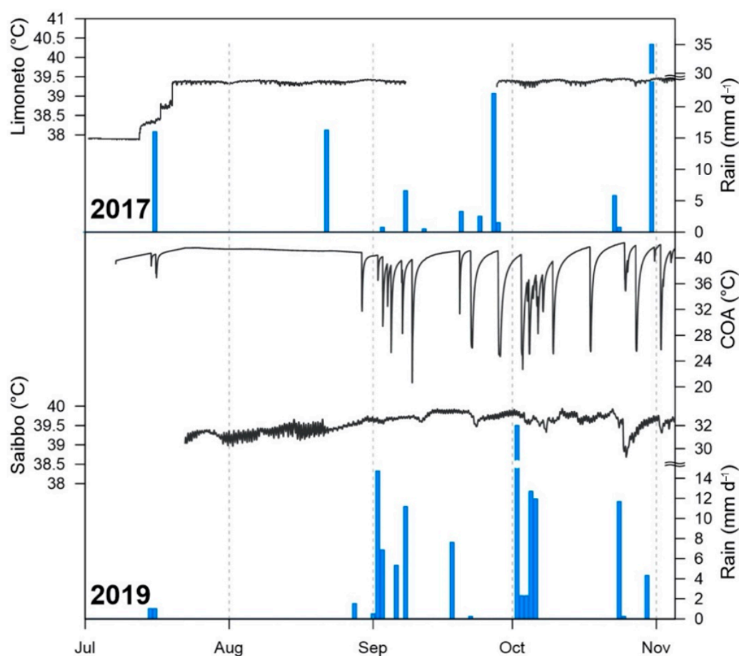
Figure 10. Hourly measures of the groundwater temperature acquired at wells LIM (2017), COA, and SAI (2019) compared with rainfall ( \text{mm d}^{-1} ). The time window covers the period of July–October of different years due to the lack of simultaneous data for the three wells.
