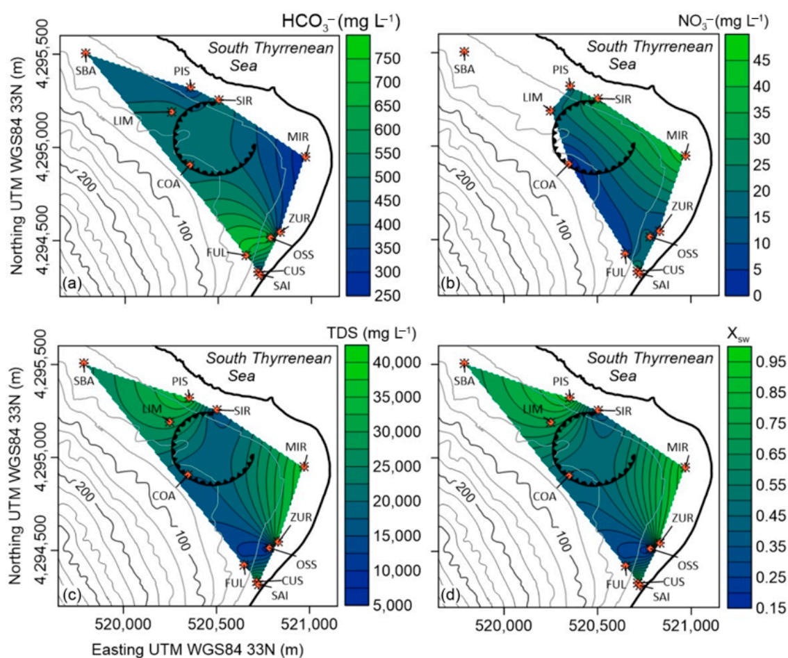
Figure 8. Concentration maps of (a) \text{HCO}_3^- , (b) \text{NO}_3^- , (c) TDS, and (d) the fraction of seawater X_{\text{sw}} .
