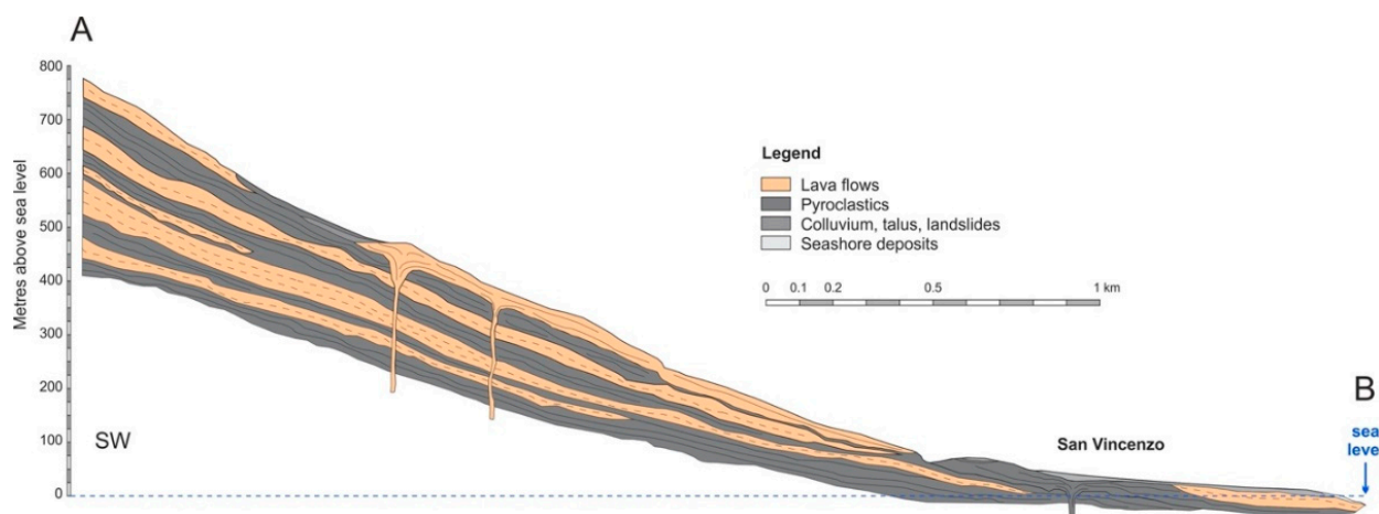
Figure 4. Schematic hydrogeological section (trace reported in Figure 2) modified after [14].
