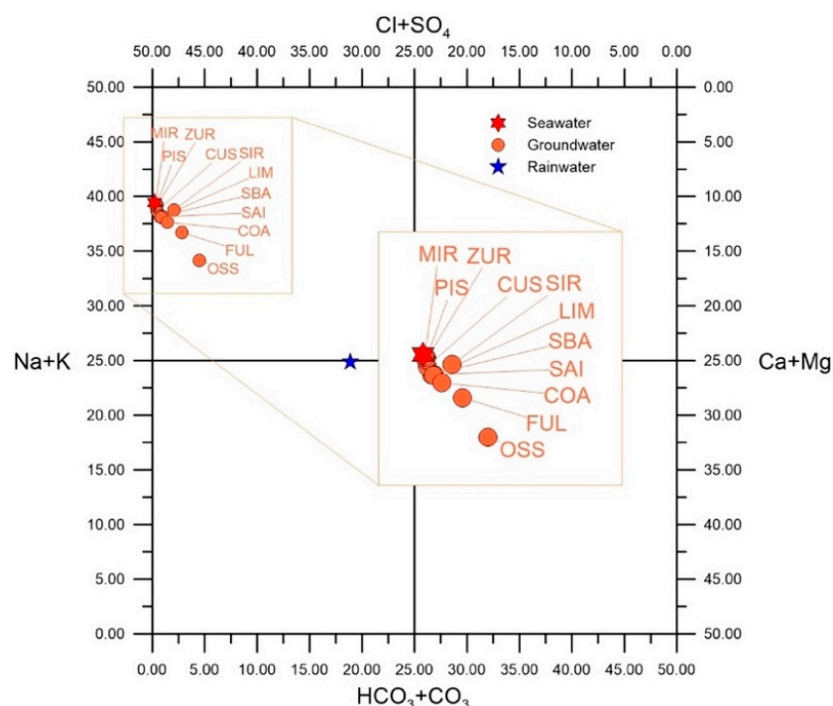
Figure 5. Plot of the average chemical composition of Stromboli groundwater in the Langelier–Ludwig diagram.
